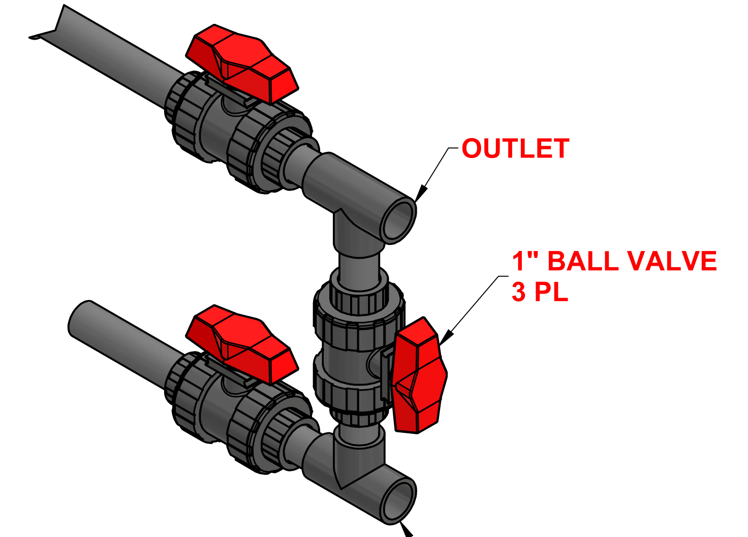
DETAIL A SCALE 0.31 : 1 OPTIONAL 3 WAY BYPASS
