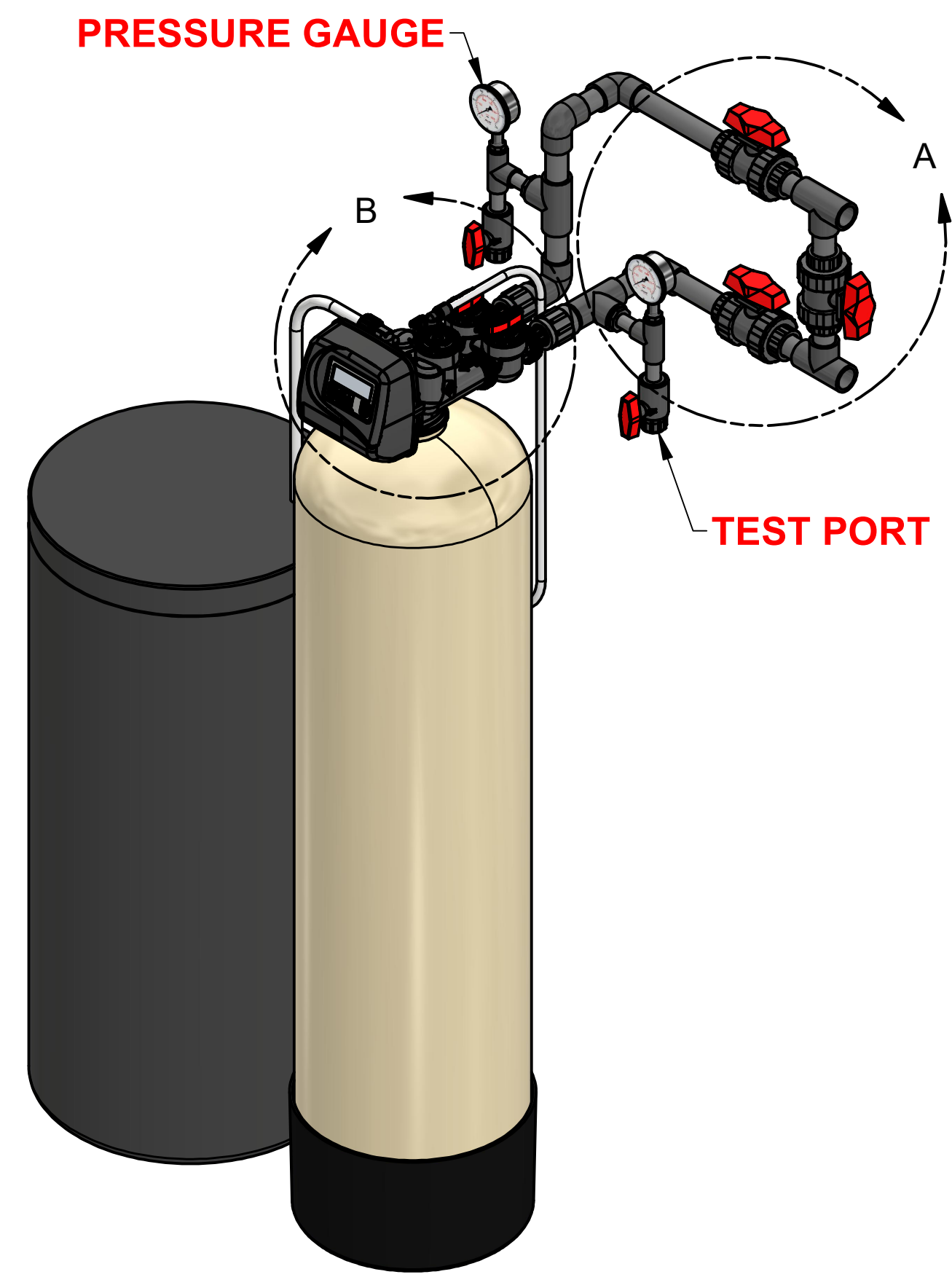
ISOMETRIC VIEW
