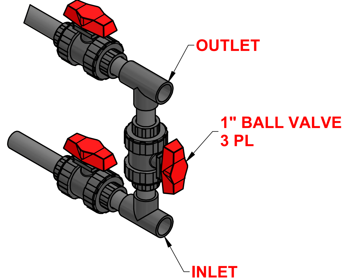
DETAIL A SCALE 1/4 OPTIONAL 3 WAY BYPASS
