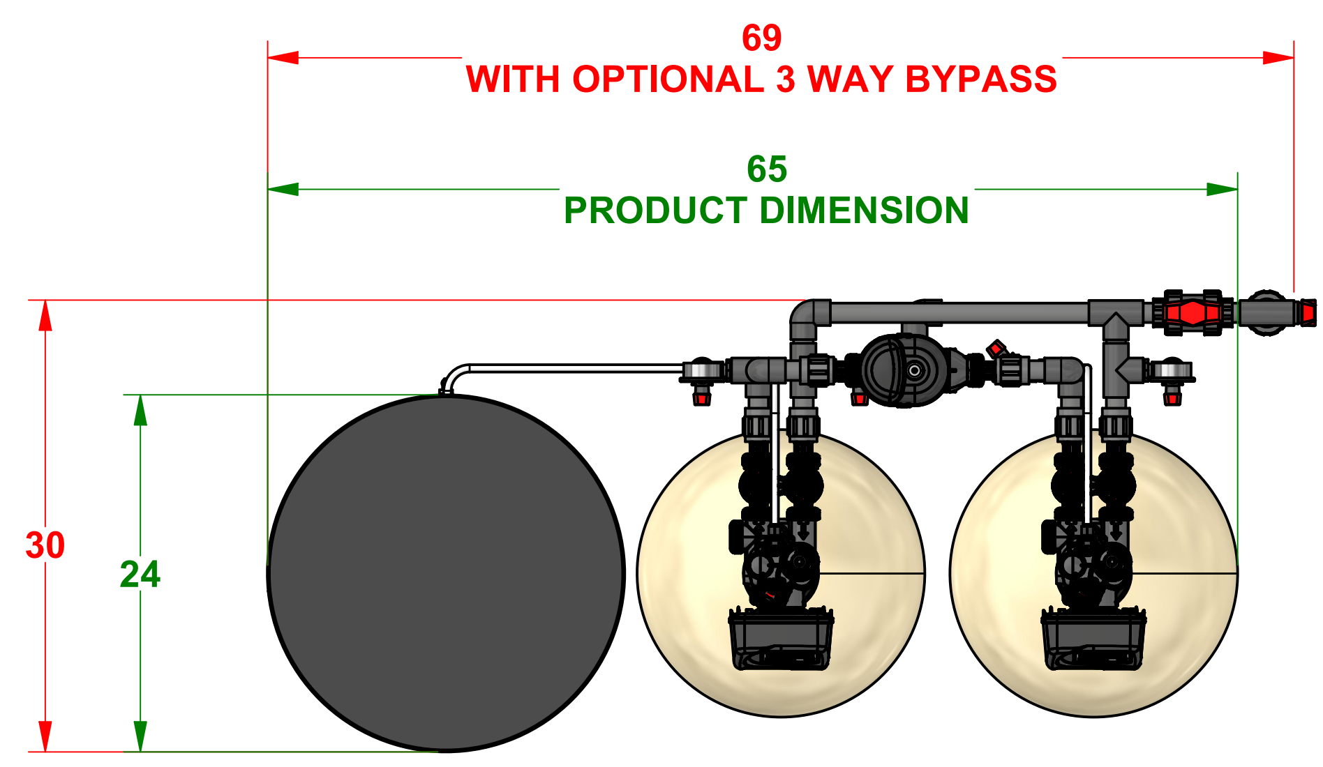
TOP VIEW
