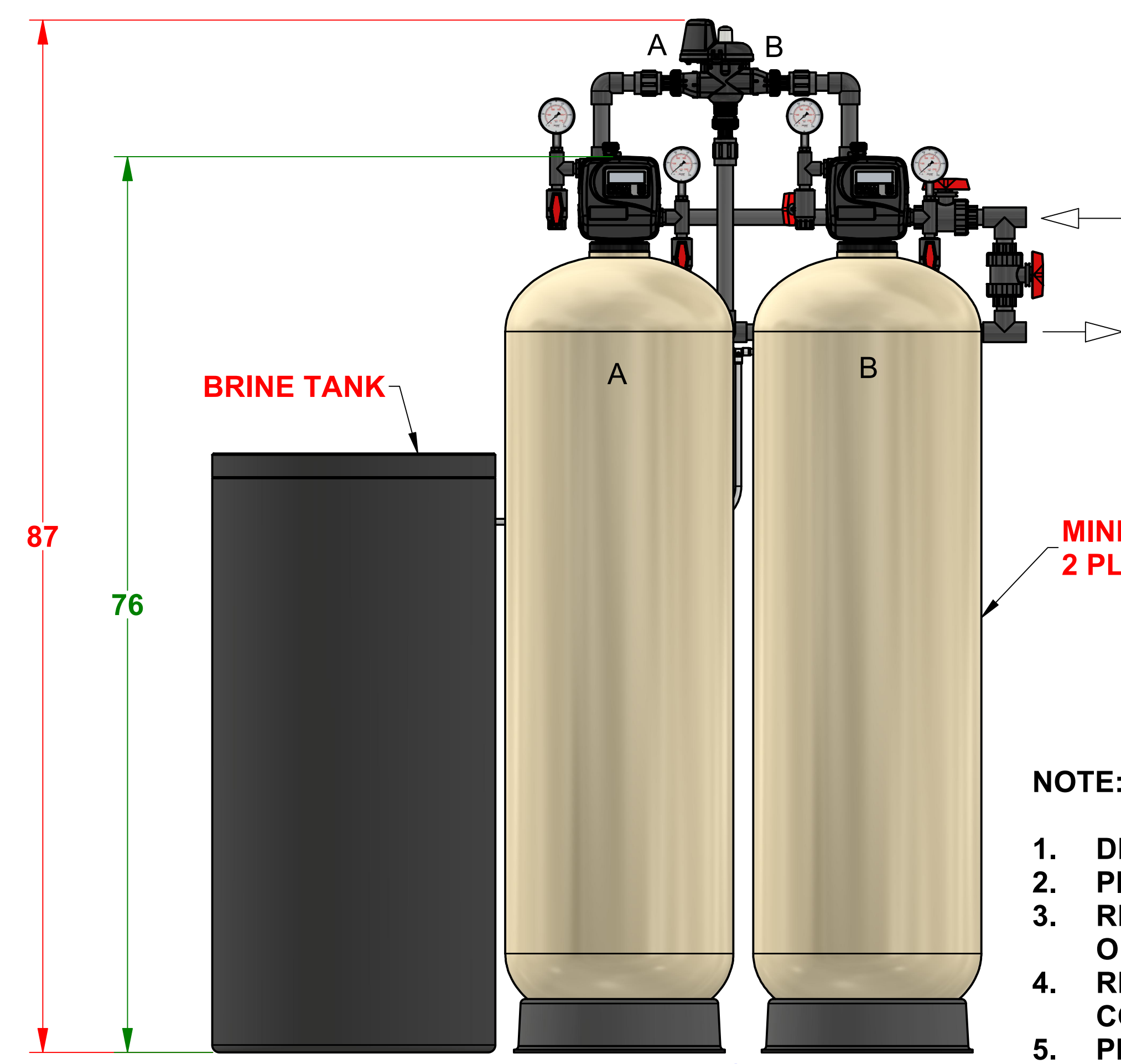
FRONT VIEW
